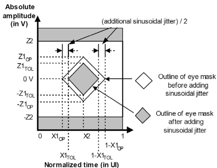
Figure 15. Receive tolerance eye mask
