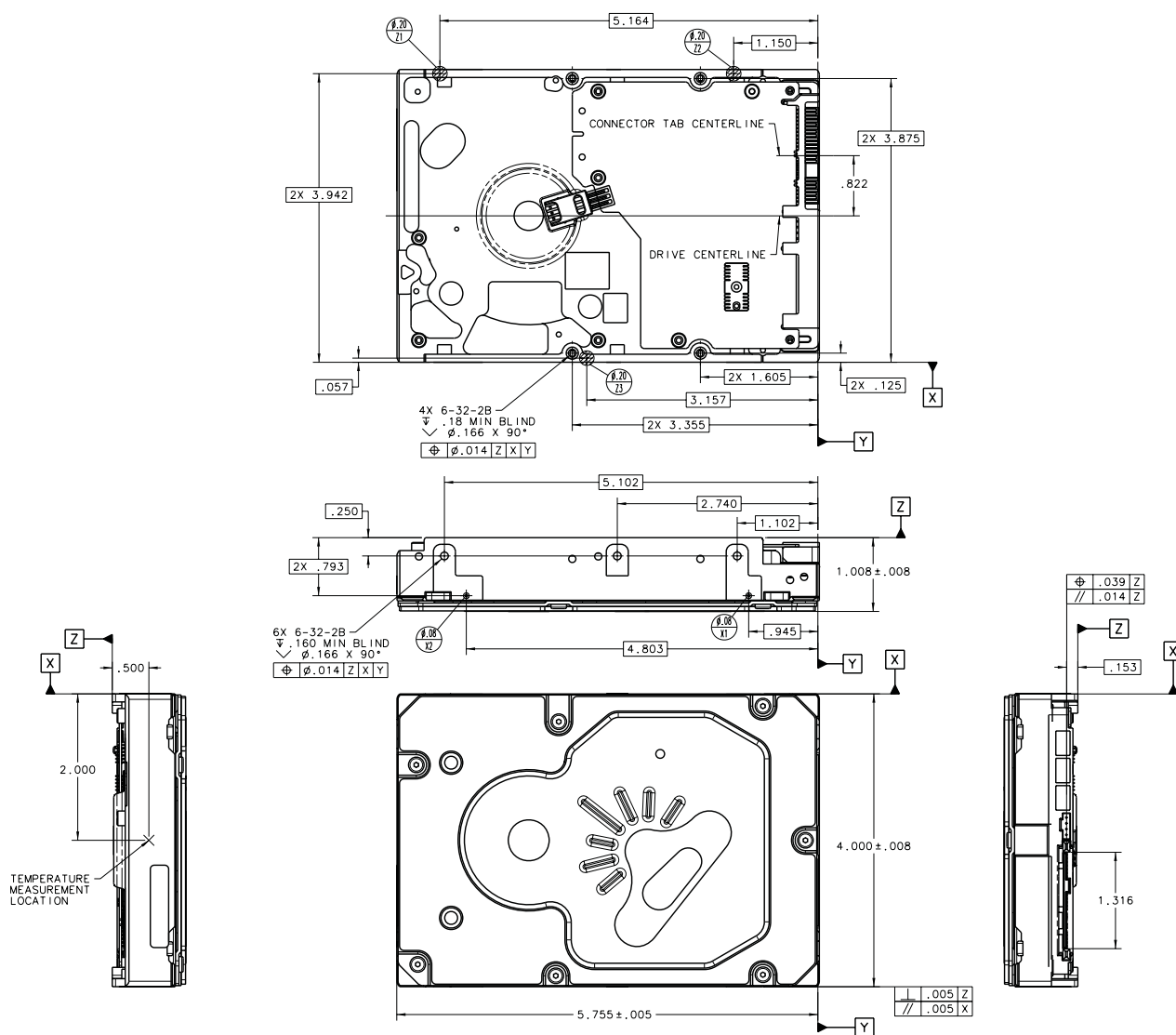
Figure 7. Physical dimensions
