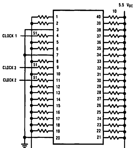
5242HR NSC810AD/883B (Dual-In-Line)
