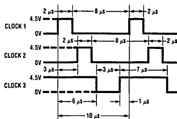
Input Clocks
