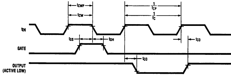
Timer Waveforms
