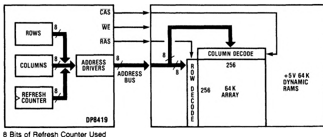
FIGURE 1c. DP8419 with 256 Row x 256 Column 64k DRAM
