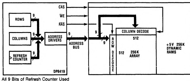
FIGURE 1d. DP8419 with 256k DRAMs
