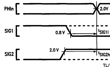
FIGURE 4-3. Timing Specification Standard (TTL Input Signals)
