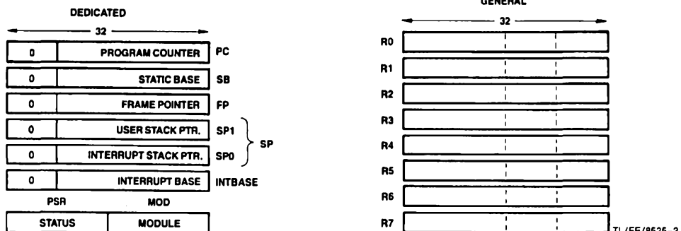
FIGURE 2-1. The General and Dedicated Registers
