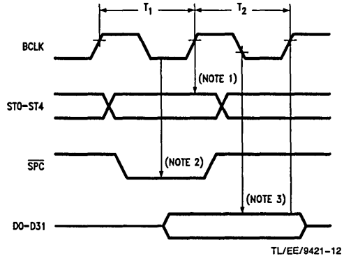
FIGURE 3-5. Slave Processor Write Cycle to FPC
