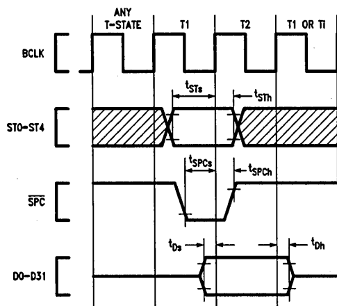
FIGURE 4-9. Write Cycle to FPC
