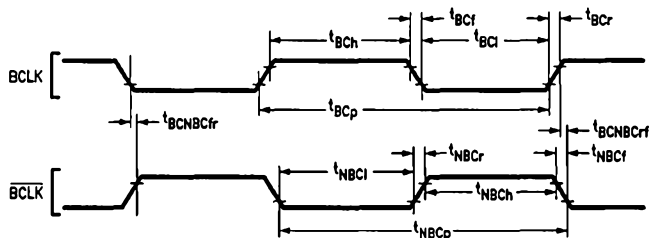
FIGURE 4-5. Clock Waveforms
