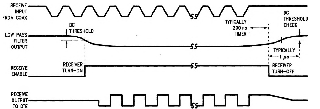
FIGURE 2. Receiver Timing
