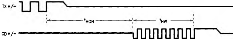
FIGURE 8. Heartbeat Timing
