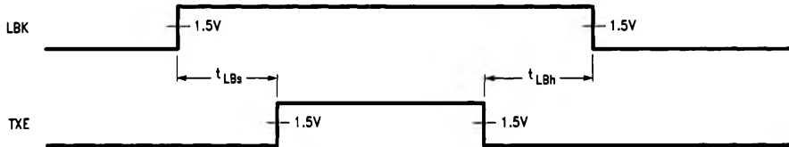
FIGURE 11. Loopback Timing
