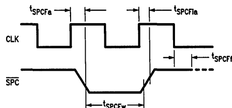
FIGURE 4-19. \overline{SPC} Pulse from FPU
