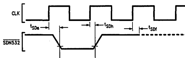
FIGURE 4-17. \overline{SDN532} Timing (NS32532 CPU)
