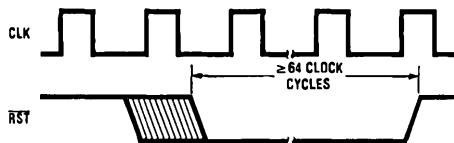
FIGURE 3-3. General Reset Timing
