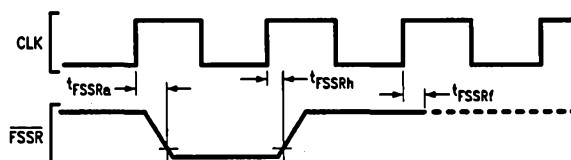
FIGURE 4-18. \overline{FSSR} Timing (NS32532 CPU)
