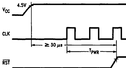
FIGURE 4-6. Power-On Reset
