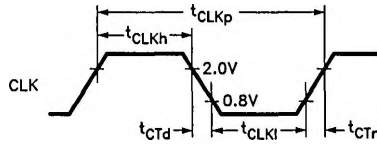
FIGURE 4-5. Clock Timing
