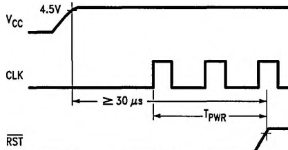
FIGURE 4-6. Power-On Reset
