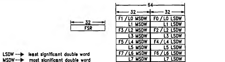
FIGURE 2-1. Register Set
