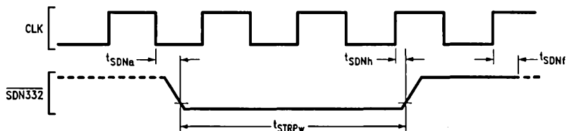
FIGURE 4-14. SDN332 (TRAP) Timing (NS32332 CPU)
