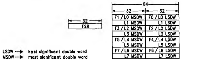
FIGURE 2-1. Register Set
