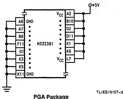
FIGURE 3-1. Recommended Supply Connections
