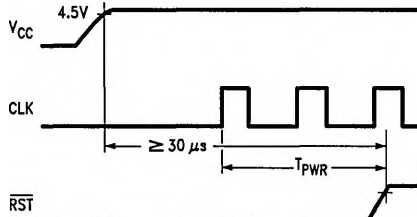
FIGURE 4-6. Power-On Reset
