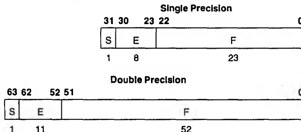
FIGURE 1-2. Floating-Point Operand Formats
