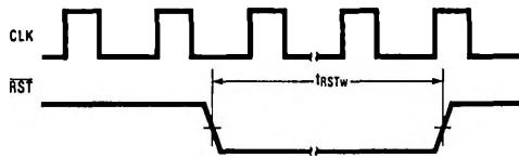
FIGURE 4-7. Non-Power-On Reset
