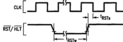
FIGURE 4-23. Non Power on Reset
