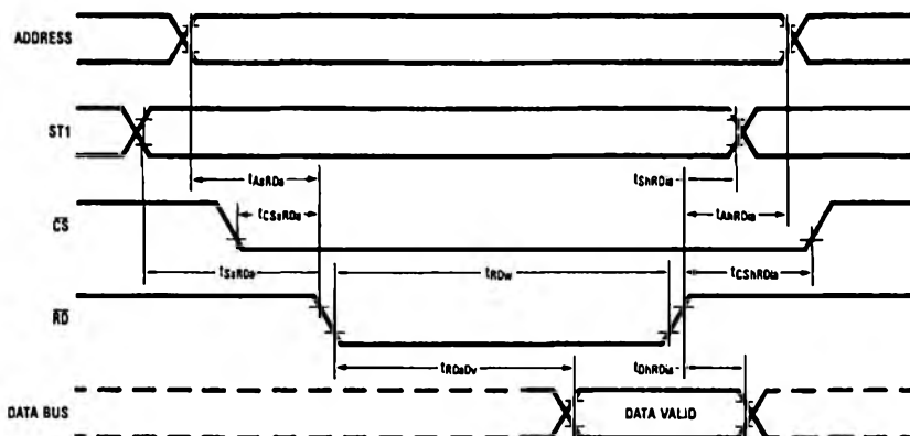
FIGURE 4-3. READ/INTA Cycle
