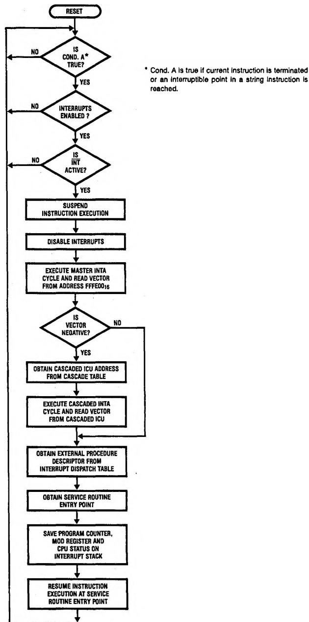
FIGURE 2-4. CPU Interrupt Acknowledge Sequence
