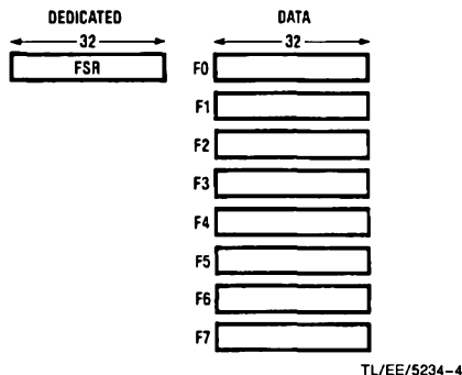
FIGURE 2-1. Register Set
