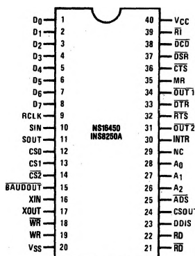
Dual-In-Line Package
