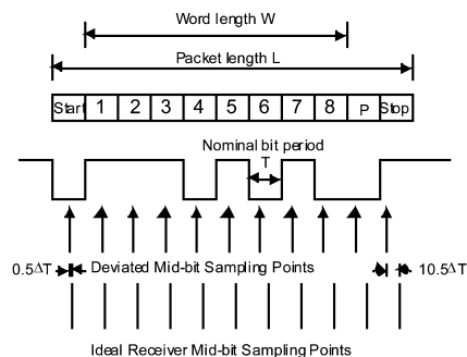
Figure 17. Deviated Baud Rate Sampling
