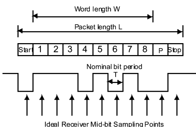
Figure 16. Nominal Mid-bit Sampling
