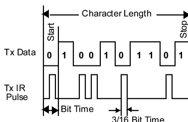
Figure 14. IrDA Data Transmission
