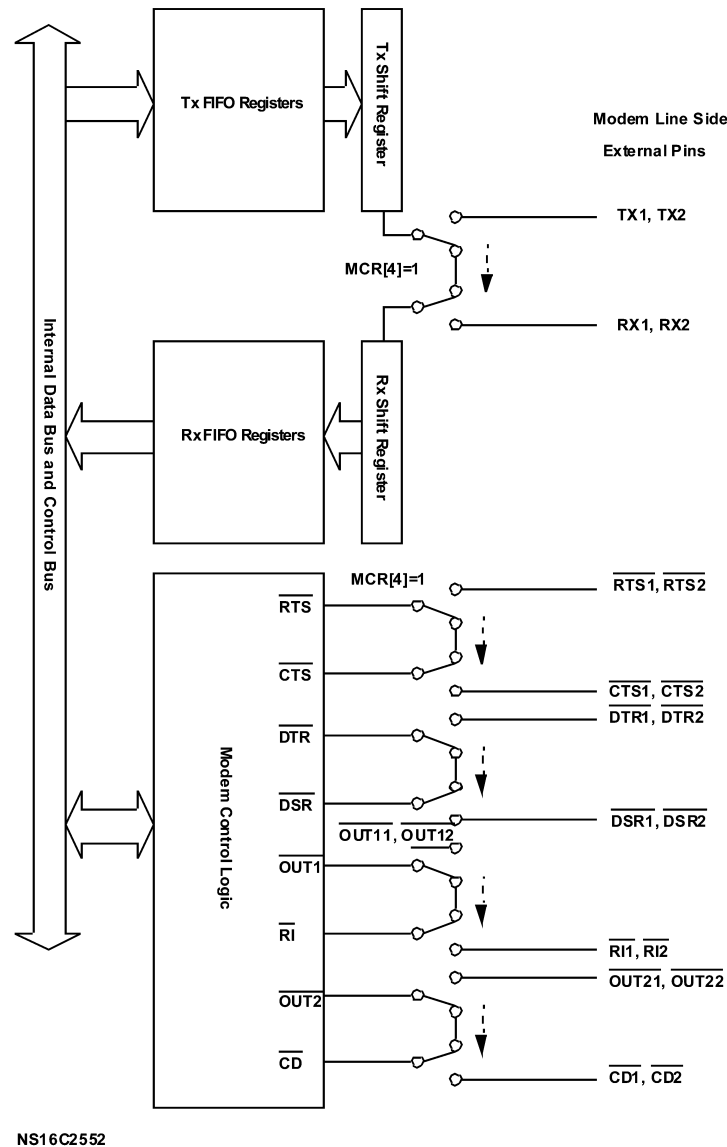
Figure 15. Internal Loopback Functional Diagram
