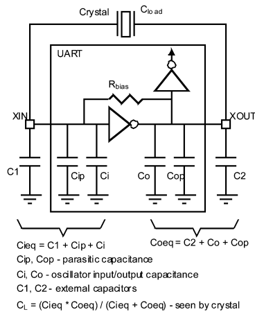
Figure 18. Crystal Oscillator Circuit
