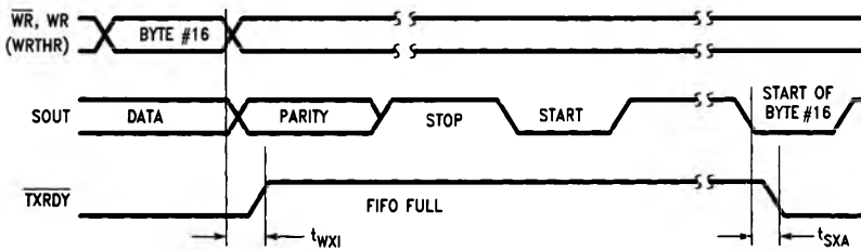
Transmitter Ready (Pin 24) FCR0 = 1 and FCR3 = 1 (Mode 1)
