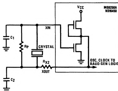
Typical Oscillator Networks
