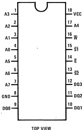
Dual-In-Line Package
