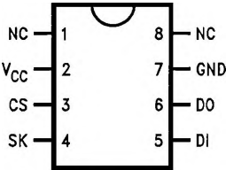
Alternate SO Pinout (TM8)
