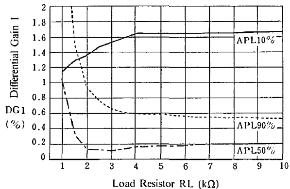
Differential Gain 1 vs. Load Resistor ( T_a = 25^\circ\text{C} )
