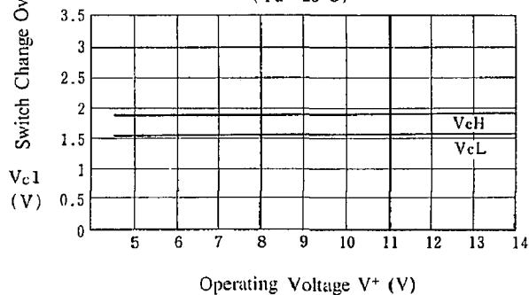
Switch Change Over 1 vs. Operating Voltage ( T_a = 25^\circ\text{C} )
