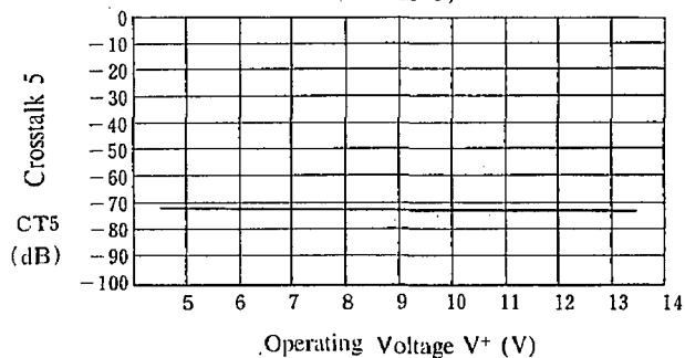
Crosstalk 5 vs. Operating Voltage ( T_a = 25^\circ\text{C} )
