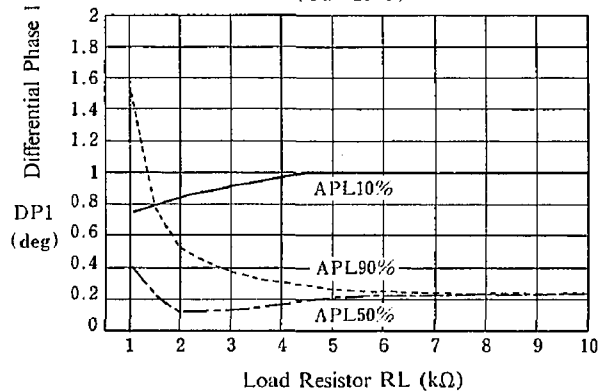
Differential Phase 1 vs. Load Resistor ( T_a = 25^\circ\text{C} )
