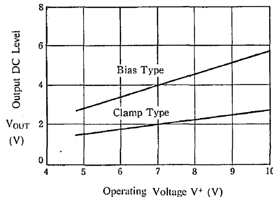
Output DC Level vs. Operating Voltage ( T_a=25^\circ\text{C} )
