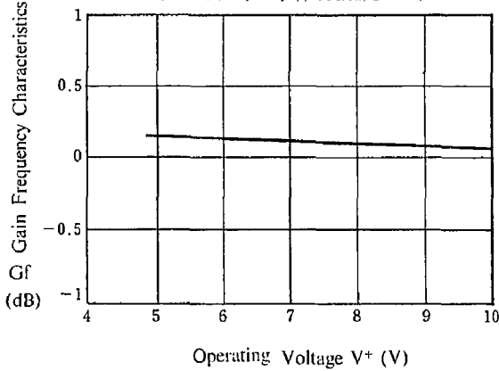
Gain Frequency Characteristics vs. Operating Voltage (Clamp Type Input) ( T_a = 25^\circ\text{C} , 1V_{p-p} , 7\text{MHz}/1\text{MHz} )
