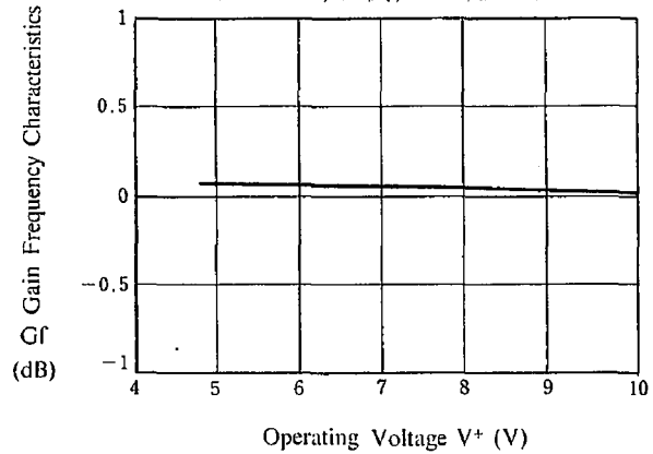
Gain Frequency Characteristics vs. Operating Voltage (Bias Type Input) ( T_a = 25^\circ\text{C} , 1V_{p-p} , 7\text{MHz}/1\text{MHz} )
