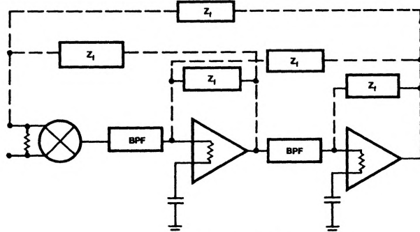
Figure 6. Feedback Paths
