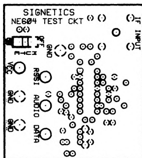
Figure 1. NE604A Test Circuit
