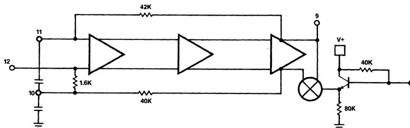
Figure 5. Second Limiter and Quadrature Detector
