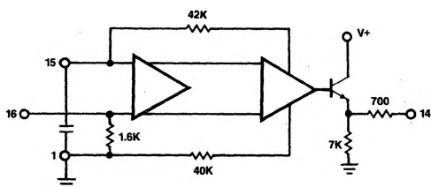
Figure 4. First Limiter Bias
