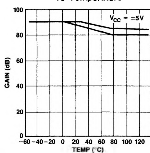
NE5570 Op Amp Gain vs Temperature
