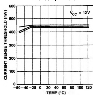
NE5570 Current Sense Comparator Threshold vs Temperature
