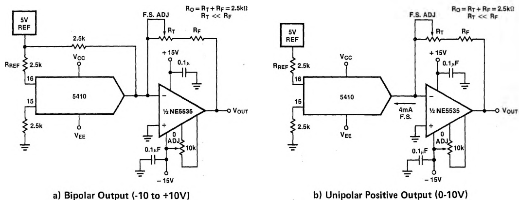
Figure 10. Voltage Output Circuits
