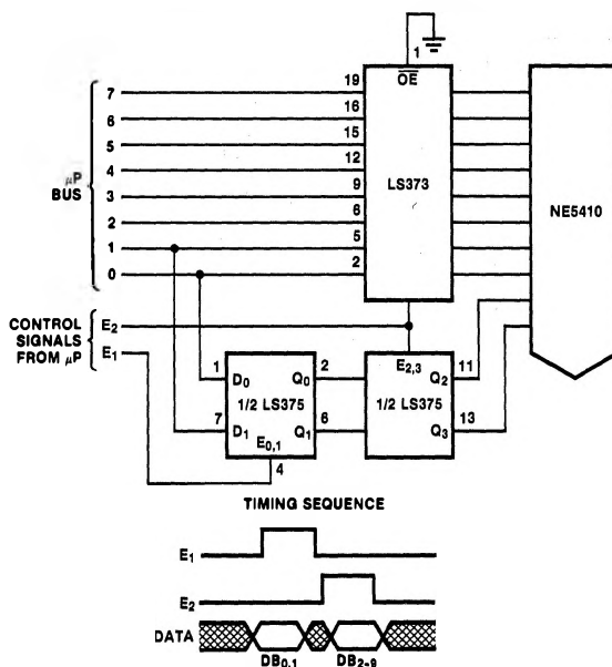
Figure 12. 8-Bit \mu P Bus Interface
