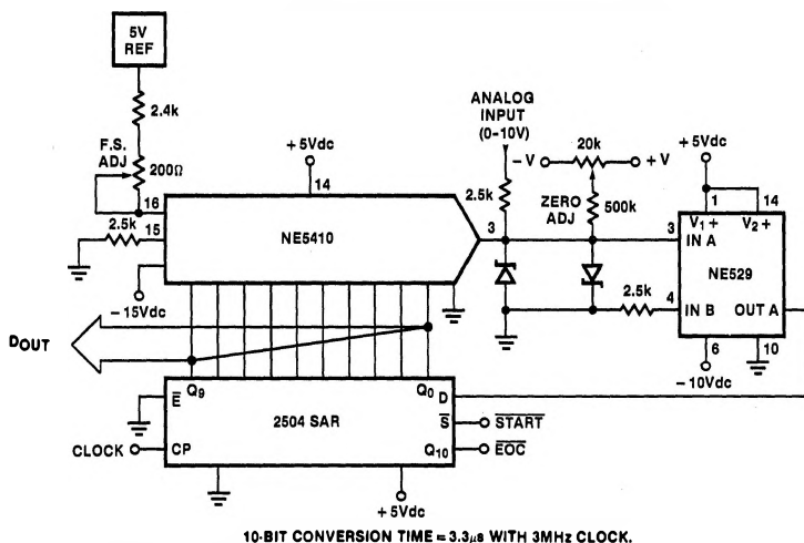
Figure 11. Successive Approximation A/D Converter
