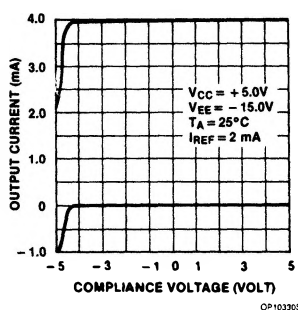
Figure 1. Output Current vs Output Compliance Voltage
