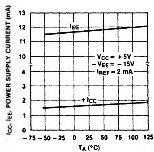
Figure 3. Power Supply Currents vs Temperature
