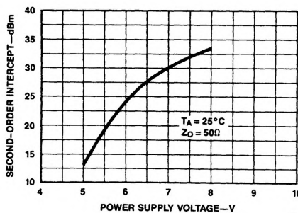
Figure 7. Second-Order Output Intercept vs Supply Voltage
