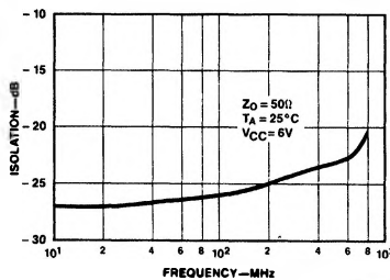
c. Isolation vs Frequency ( S_{12} )
