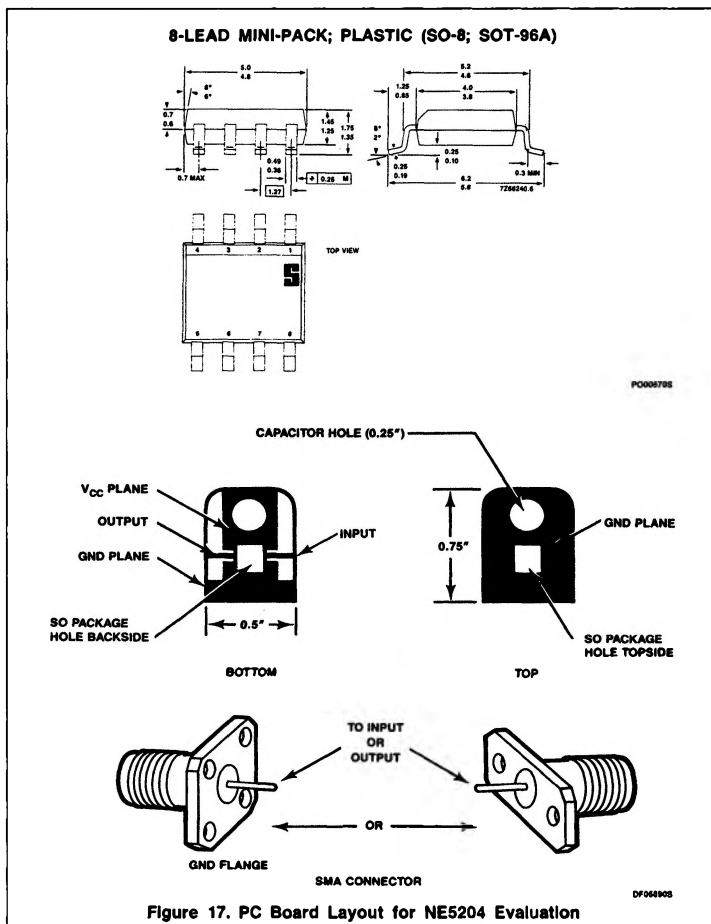
Figure 17. PC Board Layout for NE5204 Evaluation
