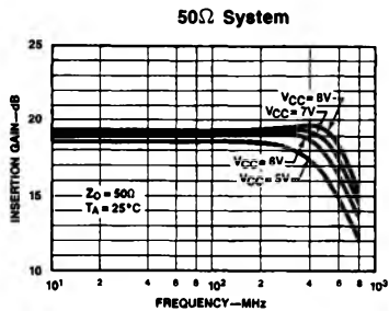
a. Insertion Gain vs Frequency ( S_{21} )
