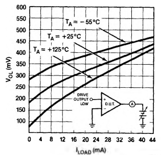
V_{SAT} vs Load Current
