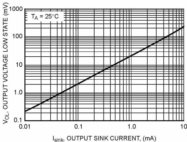
Figure 5. NCS2200 Series Output Voltage Low State vs. Output Sink Current
