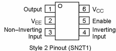
SOT23-6 (NCS2201, NCS2203)
