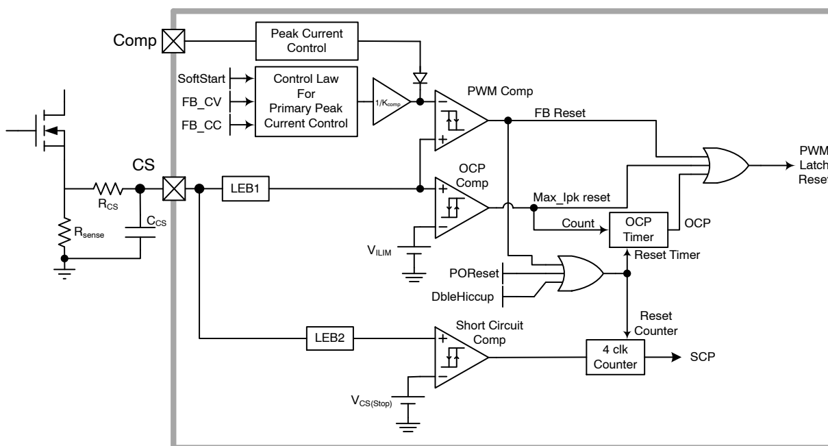
Figure 33. Current Setpoint
