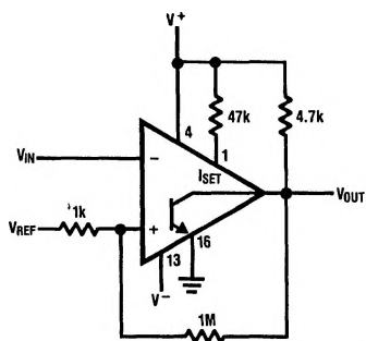
Ordinary Hysteresis
