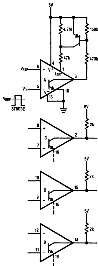
Level-Sensitive Strobe
