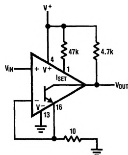
Hysteresis from Emitter
