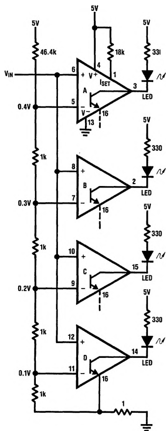
Bar-Graph Display
