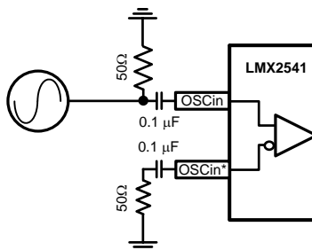
Figure 32. Single-Ended Operation
