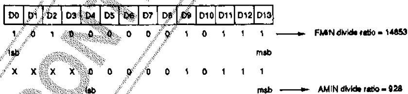
Figure 3. Divider ratio select
