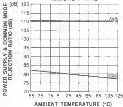
POWER SUPPLY &amp; COMMON MODE REJECTION RATIO
