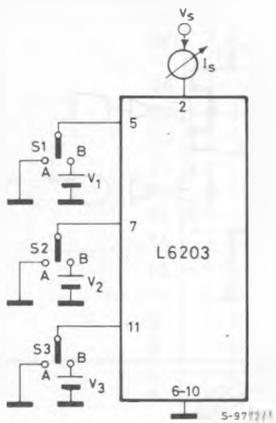
Fig. 10 - Quiescent current
