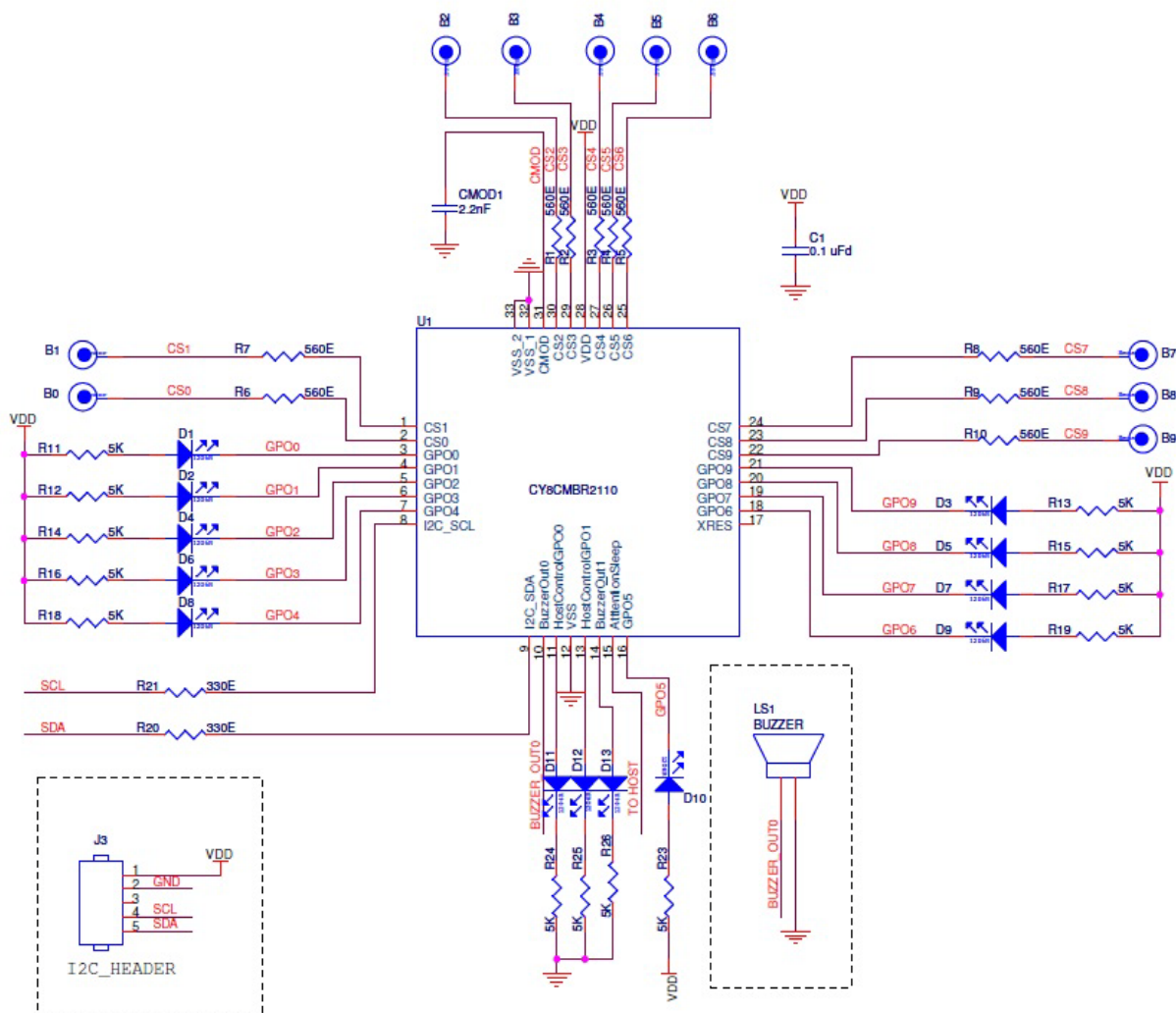
Figure 1. CY8CMBR2110 Schematic 1
