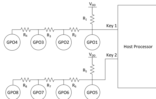
Figure 20. Analog Voltage Support for CY8CMBR2110
