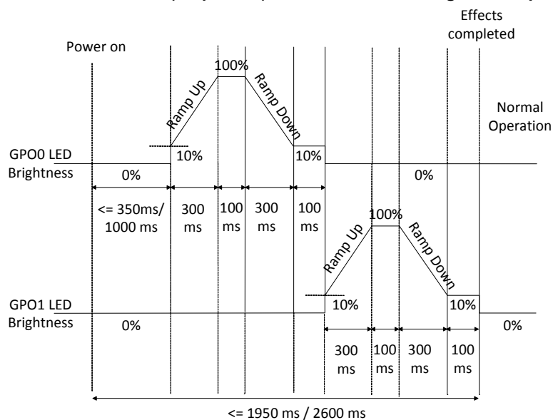
Figure 11. Example Power-on LED Effects (Sequential) with Two-Button Design and Repeat Rate = 0 [5]
