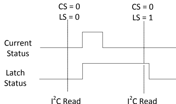
Figure 16. Latch Status Read 2
