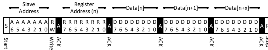
Figure 33. Host Writing x Bytes to the Device
