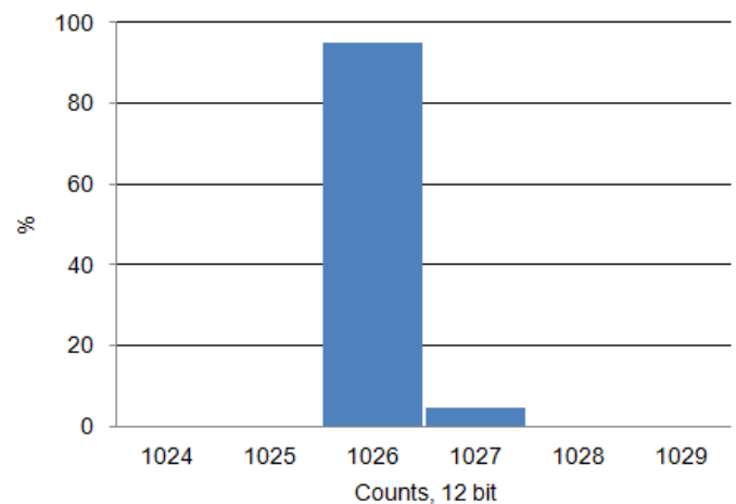
Figure 11-33. SR ADC Noise Histogram, 1000 samples, 700 kps, External Reference, V_{IN} = V_{REF}/2
