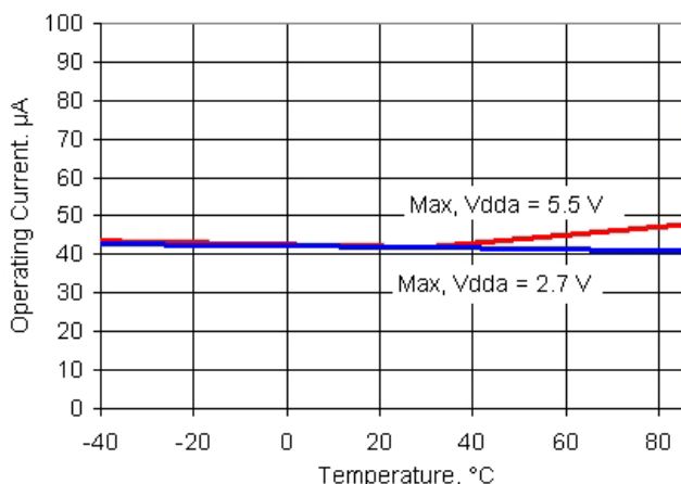
Figure 11-55. VDAC Operating Current vs Temperature, 1 V Mode, Slow Mode
