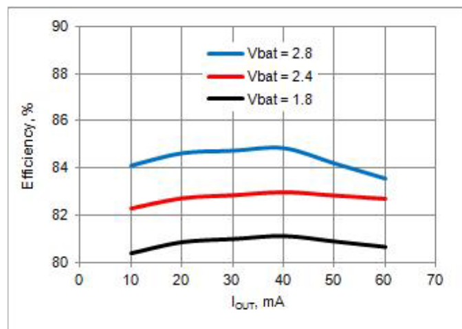
Figure 11-5. Efficiency vs I OUT V BOOST = 3.3 V, L BOOST = 10 \mu H [26]
