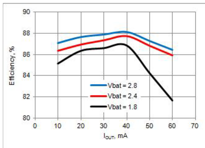
Figure 11-6. Efficiency vs I OUT V BOOST = 3.3 V, L BOOST = 22 \mu H [26]
