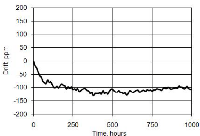
Figure 11-28. Vref Long-term Drift
