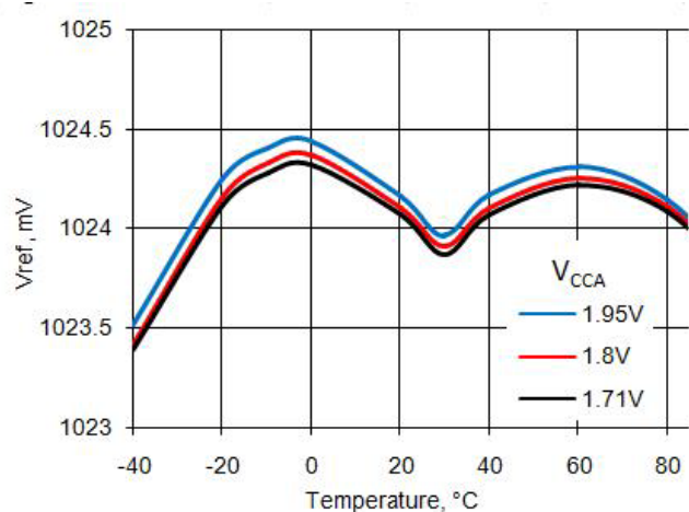
Figure 11-27. Vref vs Temperature
