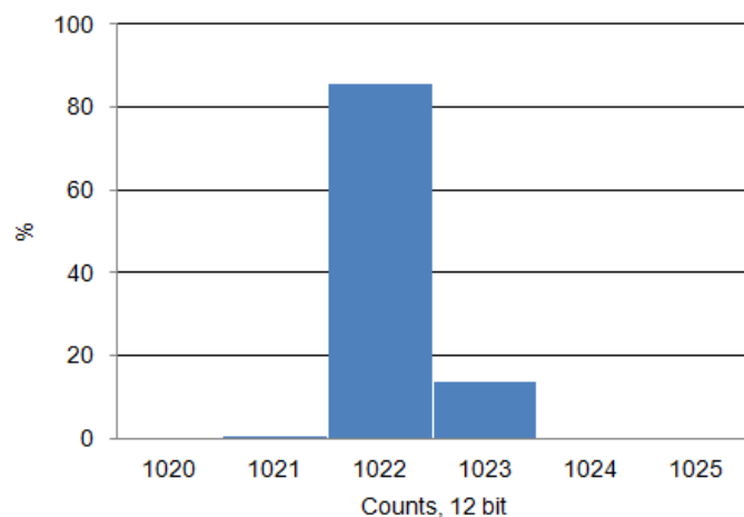
Figure 11-24. SAR ADC Noise Histogram, 1000 samples, 700 ksps, Internal Reference No Bypass, V_{IN} = V_{REF}/2
