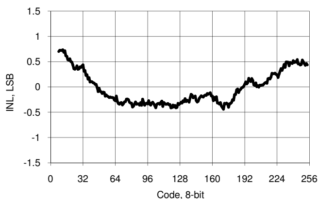
Figure 11-28. IDAC INL vs Input Code, Range = 255 \mu A, Sink Mode
