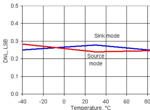
Figure 11-32. IDAC DNL vs Temperature, Range = 255 \mu A, Fast Mode
