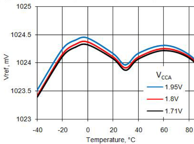
Figure 11-19. Vref vs Temperature
