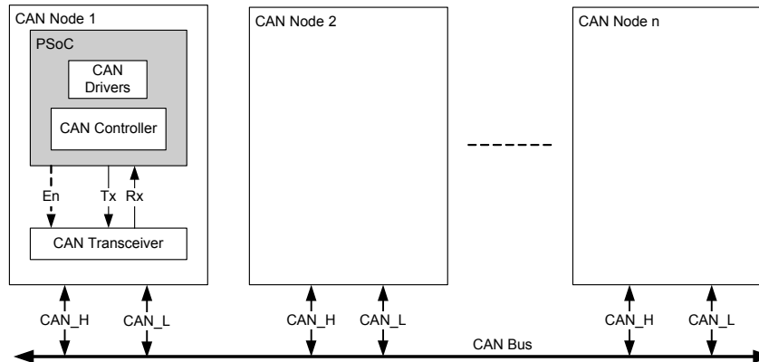
Figure 7-14. CAN Bus System Implementation
