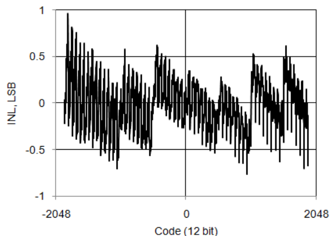
Figure 11-22. SAR ADC INL vs Output Code, Bypassed Internal Reference Mode
