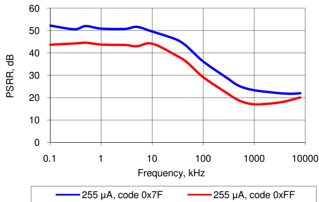
Figure 11-39. IDAC PSRR vs Frequency
