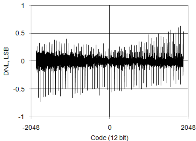
Figure 11-21. SAR ADC DNL vs Output Code, Bypassed Internal Reference Mode
