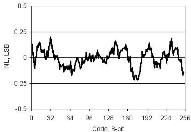
Figure 11-41. VDAC INL vs Input Code, 1 V Mode
