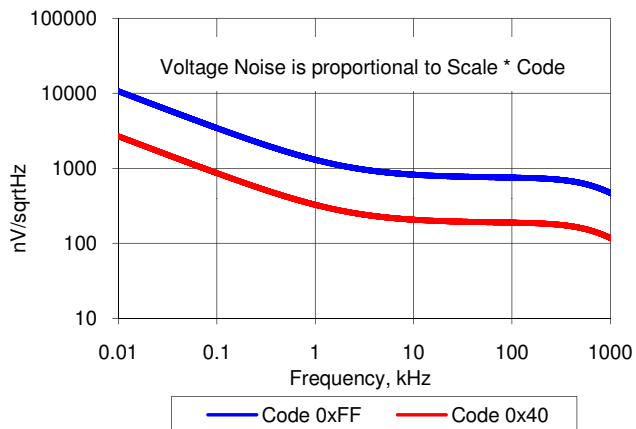
Figure 11-52. VDAC Voltage Noise, 1 V Mode, Fast Mode, V_{DDA} = 5 V
