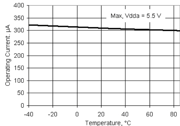
Figure 11-48. VDAC Operating Current vs Temperature, 1 V Mode, Fast Mode
