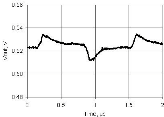
Figure 11-52. VDAC Voltage Noise, 1 V Mode, Fast Mode, V_{DDA} = 5 V
