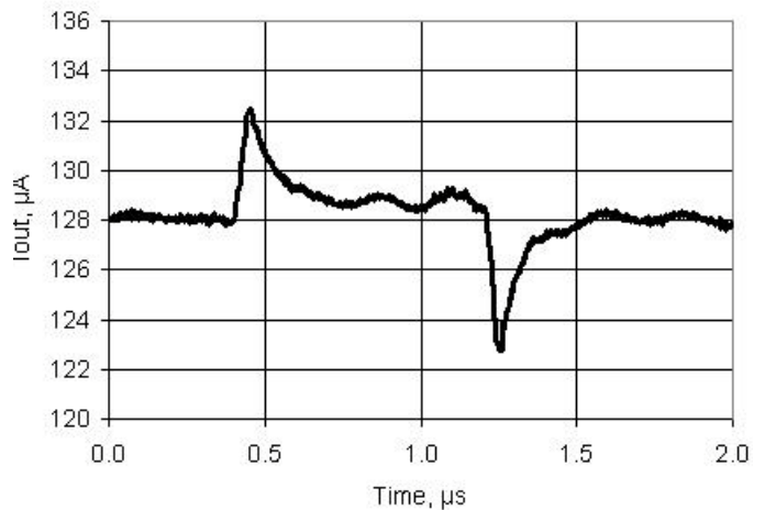
Figure 11-40. IDAC Current Noise, 255 \mu A Mode, Source Mode, Fast Mode, V_{DDA} = 5 V
