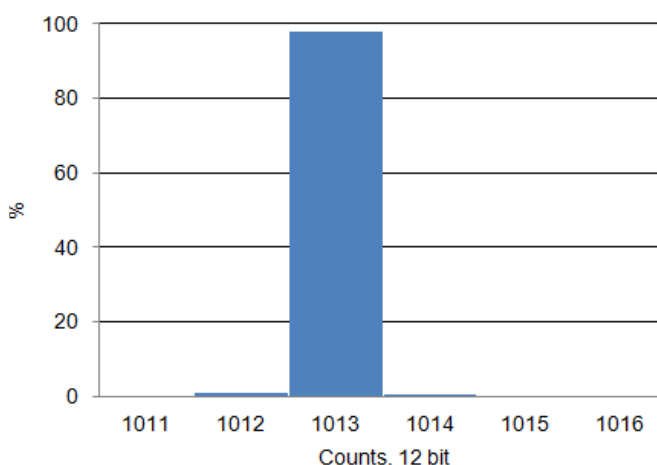
Figure 11-25. SAR ADC Noise Histogram, 1000 samples, 700 ksps, Internal Reference Bypassed, V_{IN} = V_{REF}/2
