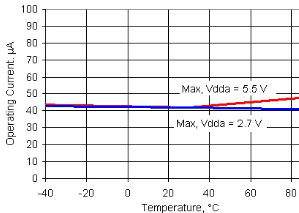
Figure 11-47. VDAC Operating Current vs Temperature, 1V Mode, Slow Mode
