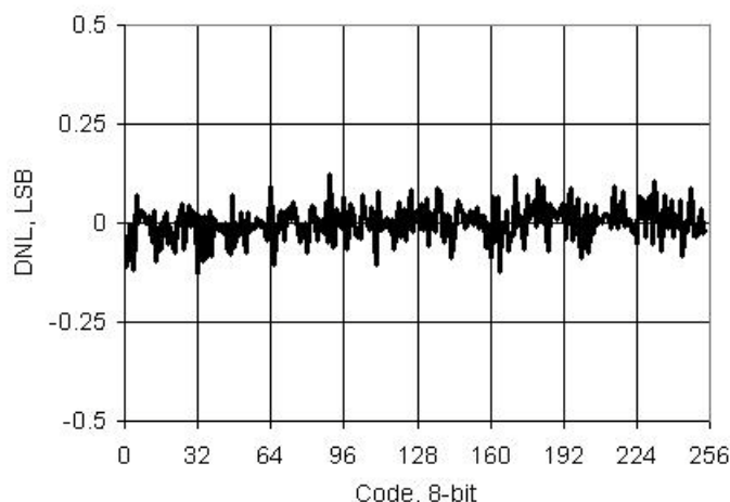
Figure 11-30. IDAC DNL vs Input Code, Range = 255 \mu A, Sink Mode
