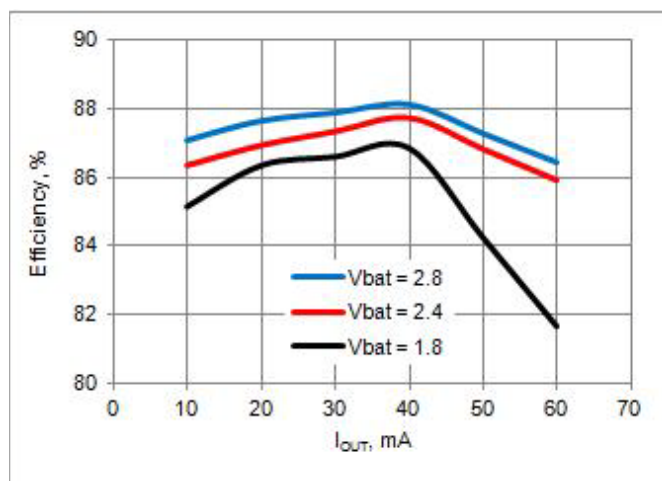
Figure 11-6. Efficiency vs I OUT V BOOST = 3.3 V, L BOOST = 22 \mu H [28]
