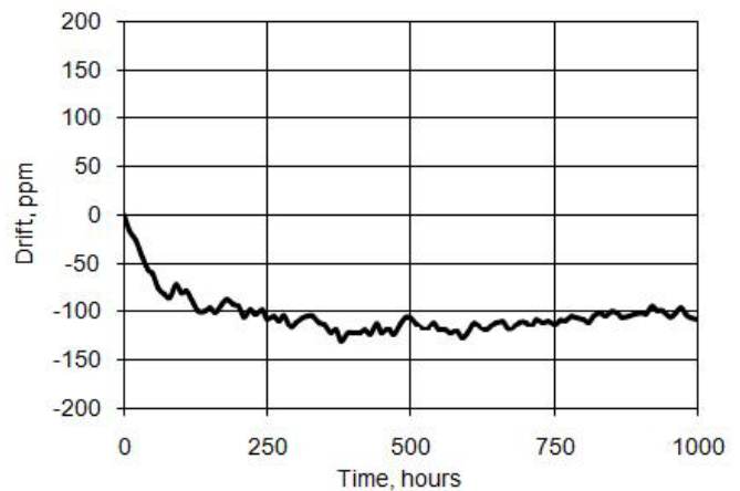
Figure 11-20. Vref Long-term Drift
