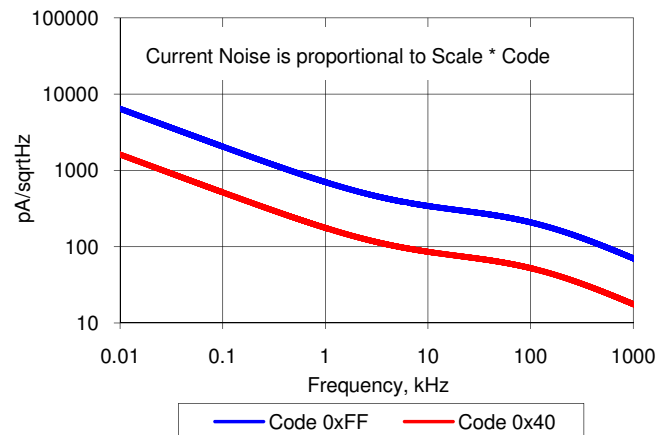
Figure 11-40. IDAC Current Noise, 255 \mu A Mode, Source Mode, Fast Mode, V_{DDA} = 5 V
