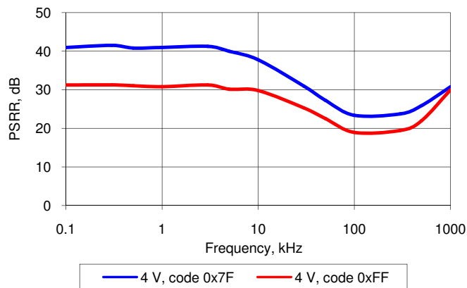
Figure 11-51. VDAC PSRR vs Frequency
