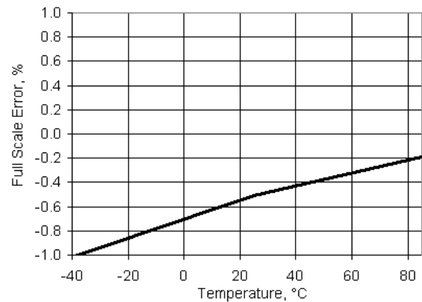
Figure 11-46. VDAC Full Scale Error vs Temperature, 4 V Mode
