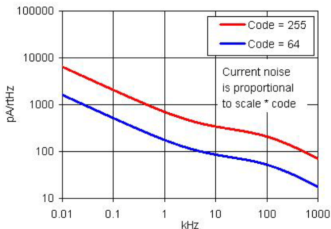
Figure 11-48. IDAC Current Noise, 255 \mu A Mode, Source Mode, High speed mode, V_{DDA} = 5 V
