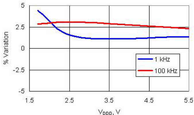
Figure 11-75. ILO Frequency Variation vs. V_{DD}
