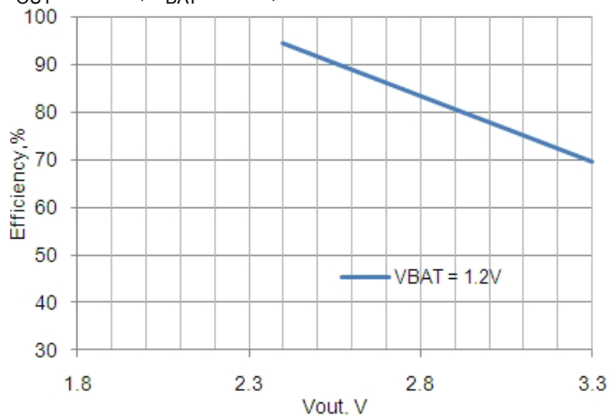
Figure 11-11. Efficiency vs V_{\text{OUT}}
