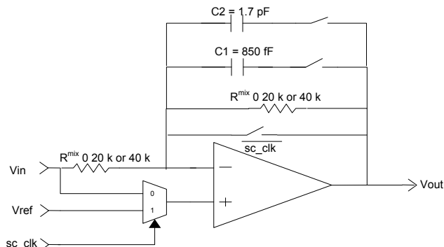
Figure 8-13. Mixer Configuration
