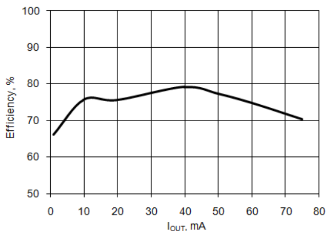
Figure 11-10. Efficiency vs I_{\text{OUT}}
