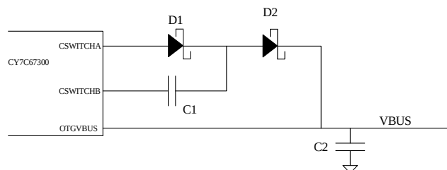
Figure 5. Charge Pump
