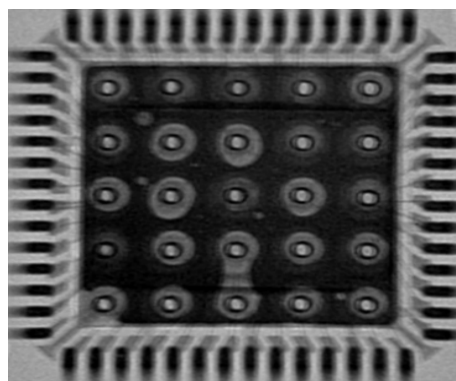
Figure 11. X-Ray Image of the Assembly
