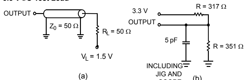
Figure 5. AC Test Loads and Waveforms
