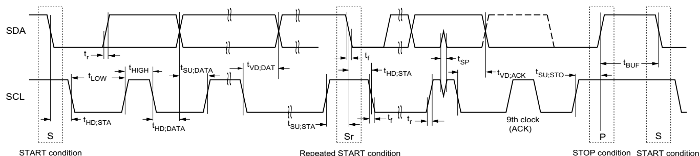
Figure 31. Timing Diagram
