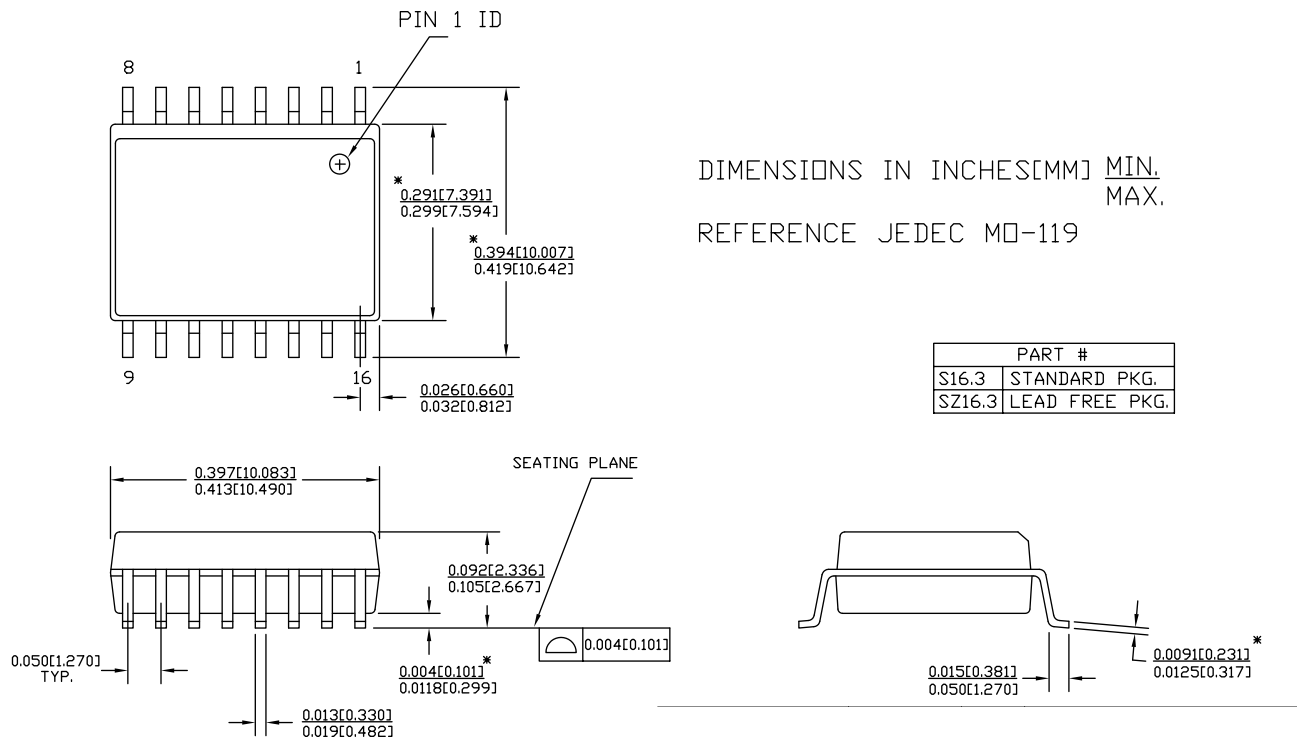
Figure 33. 16-pin SOIC (0.413 × 0.299 × 0.0932 inches) Package Outline, 51-85022
