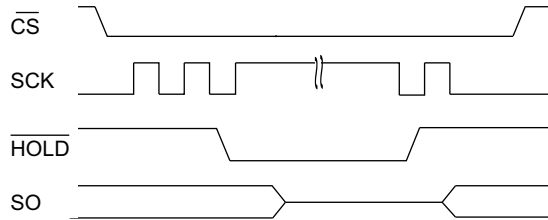
Figure 20. HOLD Operation
