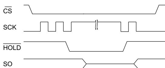
Figure 20. HOLD Operation
