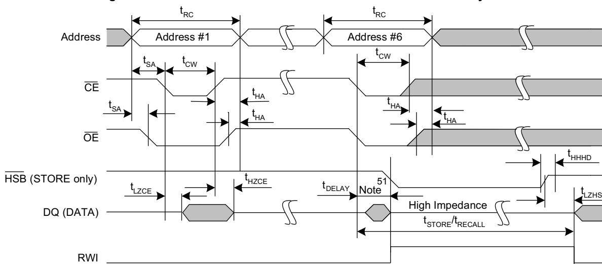
Figure 14. Autostore Enable and Disable Cycle [49, 50]
