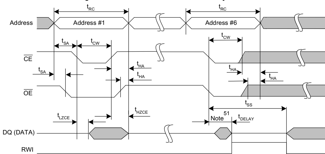
Figure 14. Autostore Enable and Disable Cycle [49, 50]
