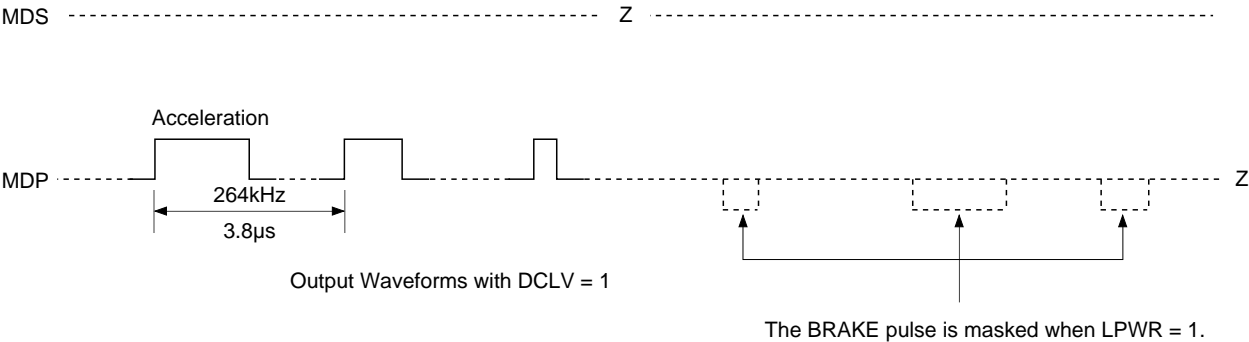
Timing Chart 1-17
