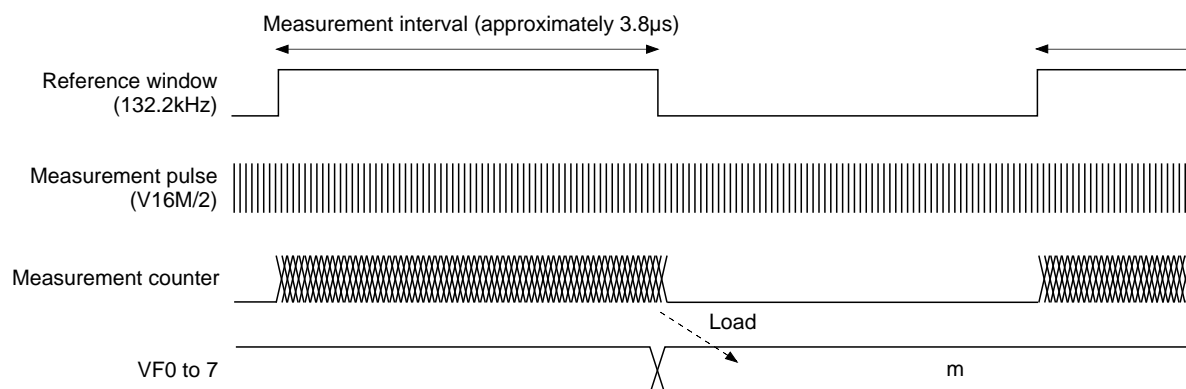
Timing Chart 2-5
