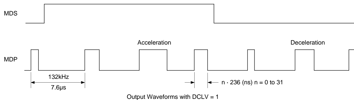
Timing Chart 1-14
